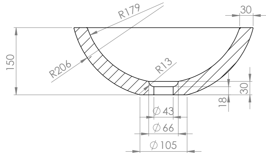
SECTION B-B
