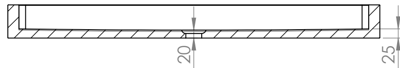
SECTION B-B
