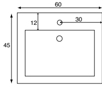
Wastafel tbv 'Fit Me' 60/70/100/120 (in centimeters)
