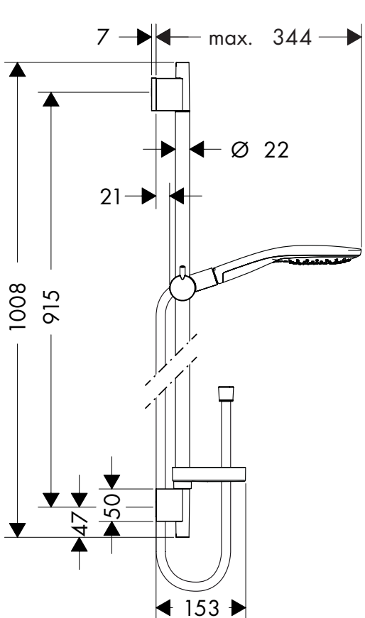
Raindance Select S 150 / Unica'S Puro Set 27803XXX
