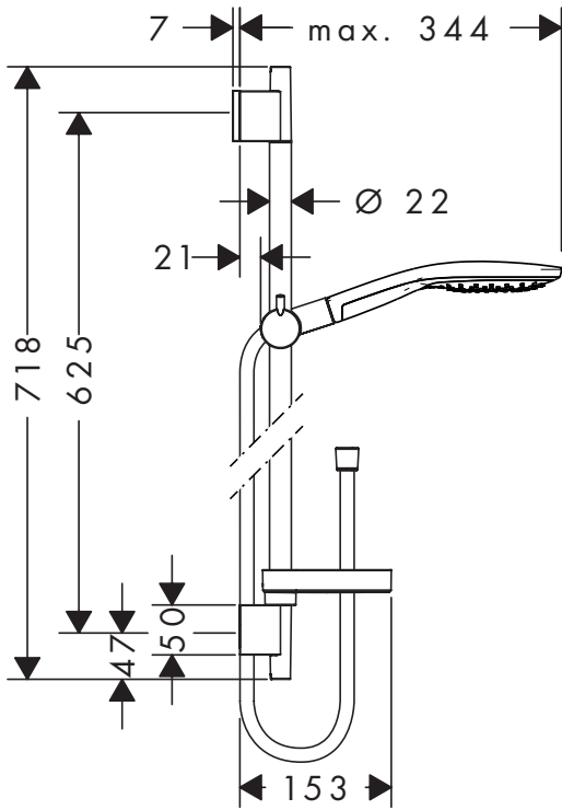
Raindance Select S 150 / Unica'S Puro Set 27802XXX
