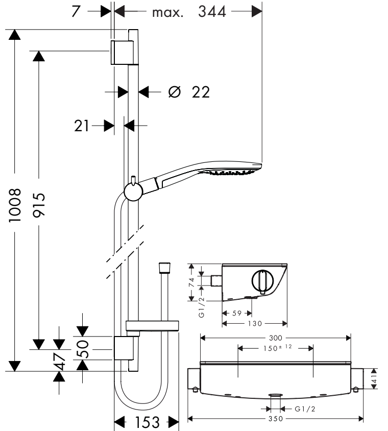
Raindance Select 150 Combi 27037XXX
