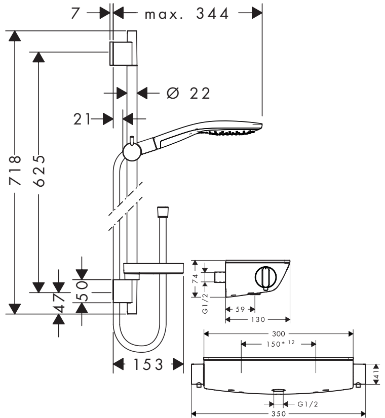
Raindance Select 150 Combi 27037XXX
