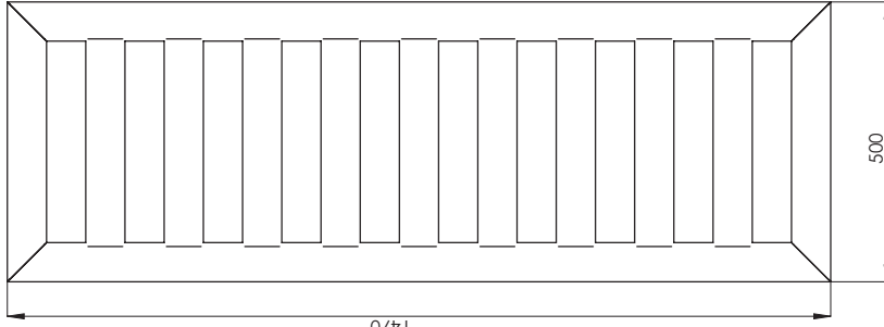
150-050 9 cross tubes
