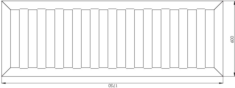
180-060 11 cross tubes
