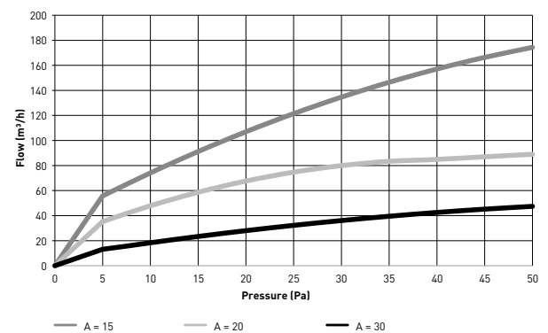
Pressure / flow curve DucoVent Basic
