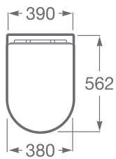
Floorstanding toilet Ref. A803061002
